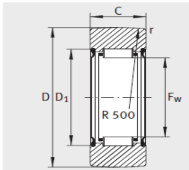
RNA22..-2RSR
