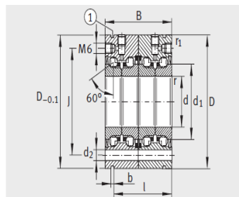
ZKLF-2RS-2AP
